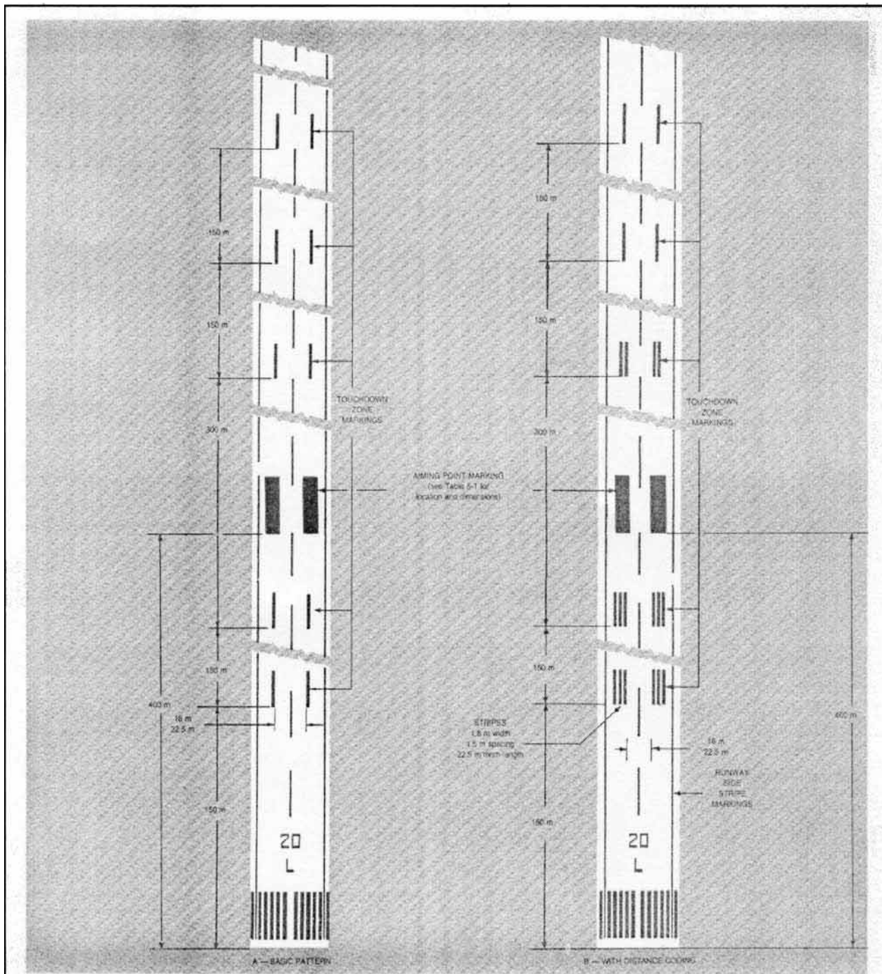
Figure 5-5. Aiming point and touchdown zone markings (illustrated for a runway with a length of 2 400 m or more)
