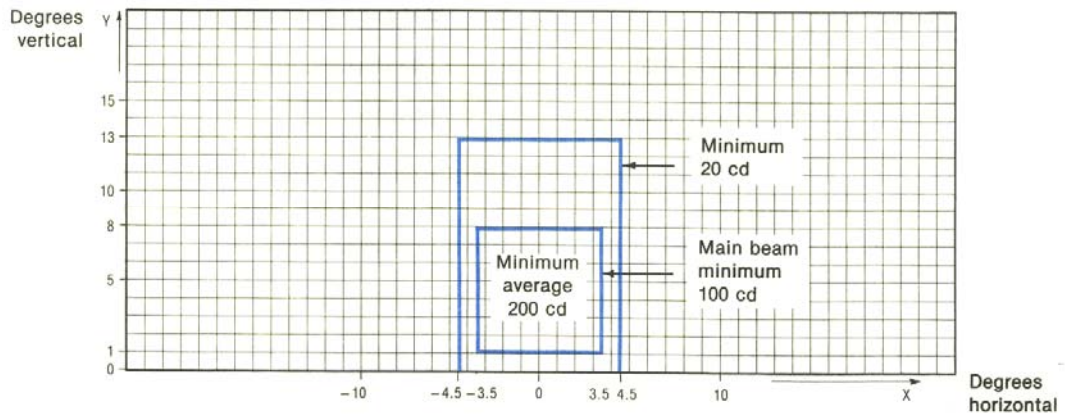
Figure 2.12. Isocandela diagram for taxiway centre line (15 m spacing) and stop bar lights in straight sections intended for use in runway visual range conditions of less than a value of 350 m where large offsets can occur and for low-intensity runway guard lights, Configuration B
